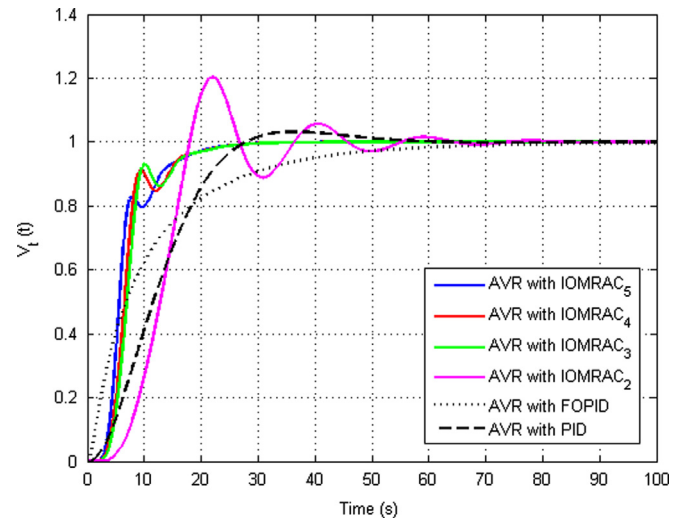
Fig. 8. Step responses of the AVR controlled by the four IOMRACs, PID and FOPID.
