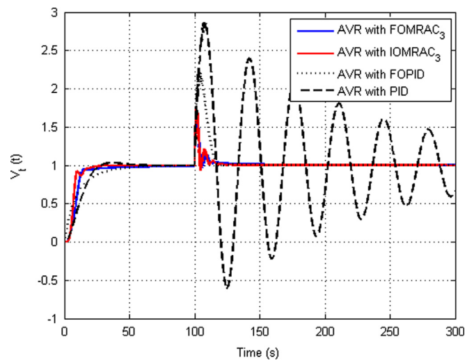
Fig. 12. Step responses of the AVR controlled by the FOMRAC 3 , IOMRAC 3 , PID and FOPID, under variations in the parameters of the generator and the exciter transfer function at t = 100 s.
