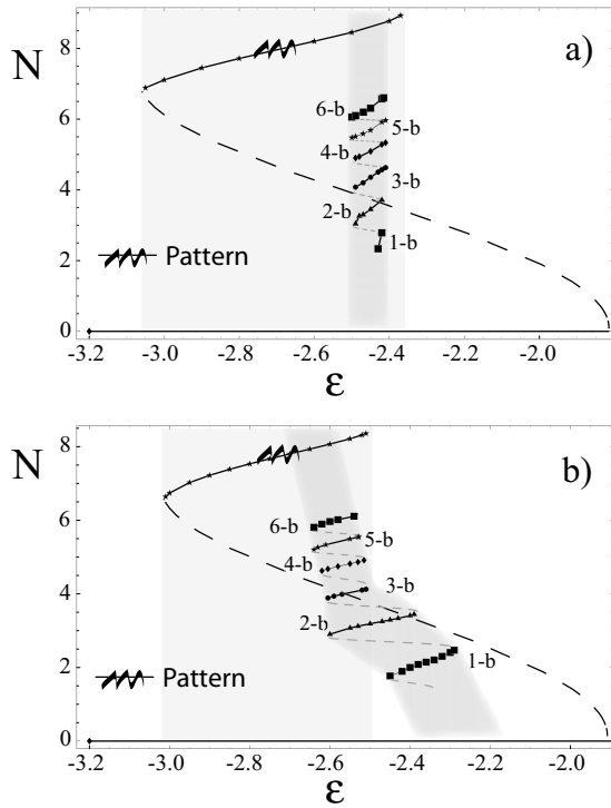
FIG. 3. Homoclinic snaking bifurcation of model (1) calculated for (a) \eta=0.1 and (b) \eta=0.4 . The horizontal axis is the bifurcation parameter \epsilon and the vertical axis is the norm ( \mathcal{N} ), where \mathcal{N} = \sqrt{\int \text{Re}(A)^2 + \text{Im}(A)^2 dx} . The solid, dashed curves stand, respectively, for the stable, unstable state. The single-bump, double-bump, and so forth, solutions are depicted by the solid lines 1-b, 2-b, etc. Points are the results of the numerical calculations.
