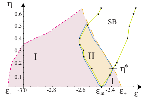
FIG. 2. (Color online) Phase diagram of the model (1) calculated for \nu=7.0 , \alpha=4.9 , and q=12 . The whole bistability region extends over areas I and II while the pinning range is region II. The dashed, dotted (red) curves represent the saddle-node bifurcation of the stable pattern with the large, respectively, small amplitude unstable pattern. The smallest localized structure, that is, the single-bump solution, is observed inside the solid (green) open curve and, after the saddle node, continues to exist in the SB region.
