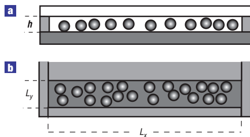
Figure 1 Schematic representation of the system. a, b , Side ( a ) and top ( b ) views of the system. In both experiments and molecular dynamic simulations, the cell geometry is: height h = 1.8d , where d is the particle diameter, length L_x and width L_y , with L_x \gg d and L_y \gtrsim d . For the experimental pressure measurements, the geometry is h = 1.7d and L_x \sim L_y .
