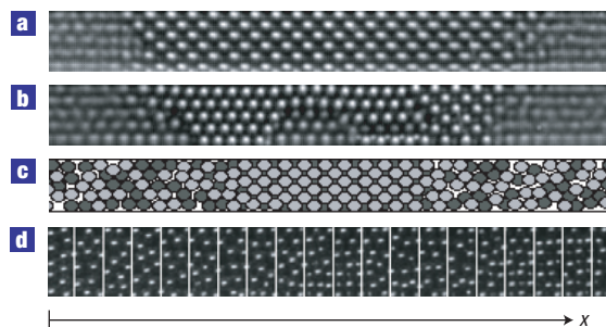
Figure 2 Solid–liquid coexistence in the confined system. a, b , Averaged images of typical crystal structures observed: vibration frequency f = 65 Hz, vibration amplitude A = 0.29d and L_y = 4.65 \pm 0.05 mm. Different symmetries are observed: a , square and b , the coalescence of two triangular solid clusters competing with a square-symmetry cluster. c , Molecular dynamic 3D simulation snapshot showing a square solid cluster coexisting with a low-density fluid, with f = 68 Hz, A = 0.29d and L_y = 4.65d . Light (dark) grey particles are in the upper (bottom) layer. In both experiment and molecular dynamics simulation \rho_o = N/N_m \approx 1 , N_m = 450 , h = 1.8d , L_x = 90d , d = 1 mm. d , Coarse-graining procedure: snapshot of the granular system in a fluid state. Vertical lines define the typical fluid elements, which are characterized by the number density \rho(x, t) and the x -longitudinal momentum density j(x, t) = \rho(v_x) . In all images, only about half of the cell is shown for clarity.
