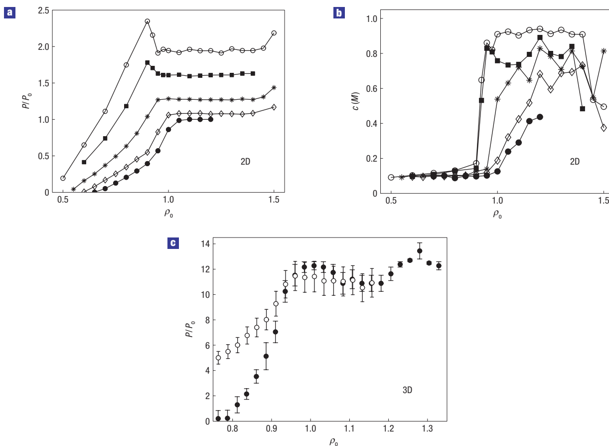
Figure 3 Pressure versus density measurements. a, b, Molecular dynamics pressure measurements and contrast order parameter for a confined hard-disc (2D) system. These results show that the pressure plateau is concomitant with the solid–liquid phase separation. Pressure is normalized by P_0 = \rho_{\text{mx}} v_0^2 , where \rho_{\text{mx}} is the maximum mass density that fits in a monolayer and v_0 = 2\pi fA is the vibration's maximum velocity. Simulation parameters are 40 \leq N \leq 400 , L_x = 400d , h = 1.8d , A = 0.35d , f = 10\sqrt{g/d}/\pi , \mu_s = \mu_d = 0.05 , \epsilon_{pw} = 1 , \epsilon_{pp} = 0.996 (open circles), 0.9 (filled squares), 0.8 (asterisks), 0.6 (open diamonds) and 0.4 (filled circles), where \mu_{s,d} stands for static or dynamic friction coefficients and \epsilon_{pw} ( \epsilon_{pp} ) stands for particle–particle (particle–wall) restitution coefficients. c, Experimental (filled circles) and molecular dynamics (open circles) results obtained in 3D shallow systems. Set-up: d = 3 mm, L_x = 18.5d , L_y = 19d , h = 1.7d , f = 70 Hz and A = 0.034d . A constant-pressure region is observed in the range \rho_0 = 1\text{--}1.3 for experiments, and \rho_0 = 1\text{--}1.15 for molecular dynamics. The experimental error bars are due to a combination of uncertainties associated with the angle measurement as well as standard deviations in other factors affecting the overall granular pressure. For the molecular dynamics results, the errors are the standard deviation from the mean.
