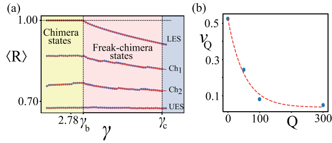
Fig. 4. The transition from chimera state to freak-chimera state. (a) Temporal Average of the global Kuramoto order parameter for different extended states. The symbols LES, UES, Ch 1 and Ch 2 account for lower extended, upper extended, and chimera states, respectively. (b) Power law exponent \nu_Q as a function of the number of oscillators in the upper extended domain Q .
