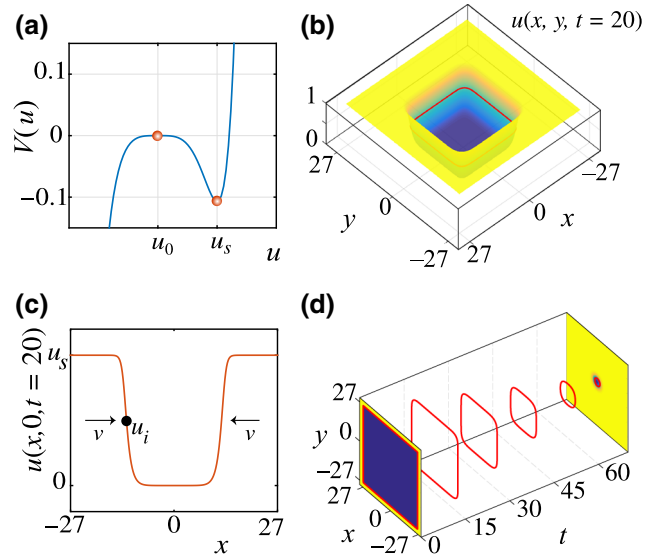
FIG. 2. Front propagation in the reaction diffusion model, Eq. (2), with K_1 = K_2 = 1 and D = 1.0 . (a) Potential of the free energy \mathcal{F} of the model in Eq. (2). u_0 and u_s account for the unstable and stable equilibria. (b) Two- and (c) one-dimensional profile of water vapor concentration u(\vec{r}, t) at a given time. (d) Temporal sequence of the evolution of the interface characterized by u = u_i (red).
