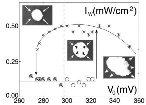
FIG. 3. Bistability and front propagation in the I_w vs V_0 plot. Circles, dark state with writing light off; stars, white state with writing light off; crosses, white state with writing light on.
