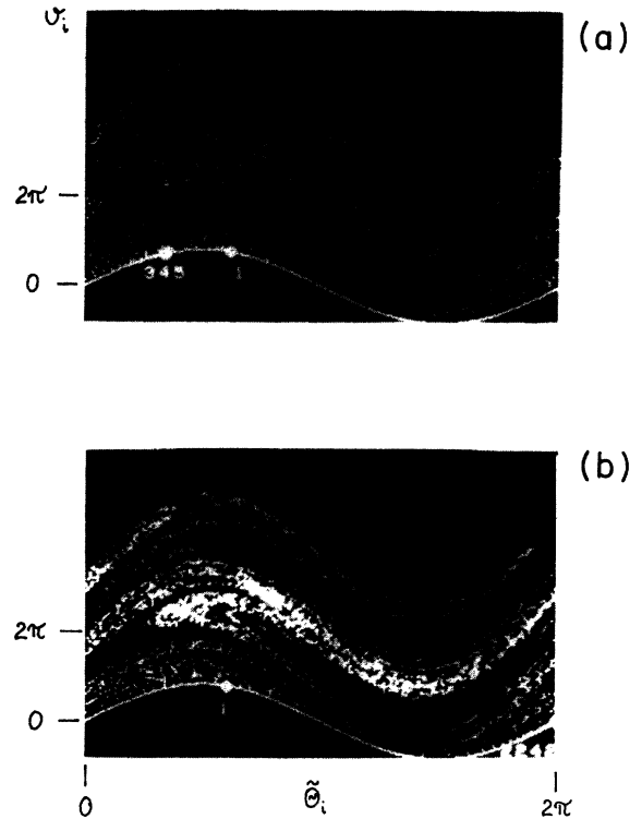
FIG. 5. Sensitivity on the initial conditions represented in the (\bar{\theta}_i, \vartheta_i) plane for K=0.86 , \lambda=4.93 . The initial point is (\bar{\theta}_1, \vartheta_1) = (\bar{\theta}_1^{(0)} + \Delta, \vartheta_1^{(0)}) . (a) \Delta = 5 \times 10^{-3} ; (b) \Delta = 10^{-3} . The initial ( i=1 ) and final points ( i=345 and 2242 ) of the trajectories are indicated in the plot with squares.
