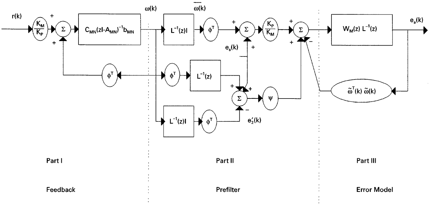
Figure 2. Decomposition of adaptive system
