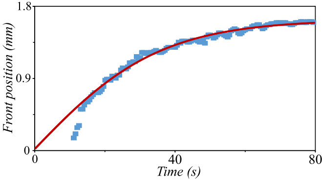
FIG. 9. Temporal wall location evolution in 1D configuration x_0(t) : ■ experimental points, — fit with hyperbolic tangent expression (19).
