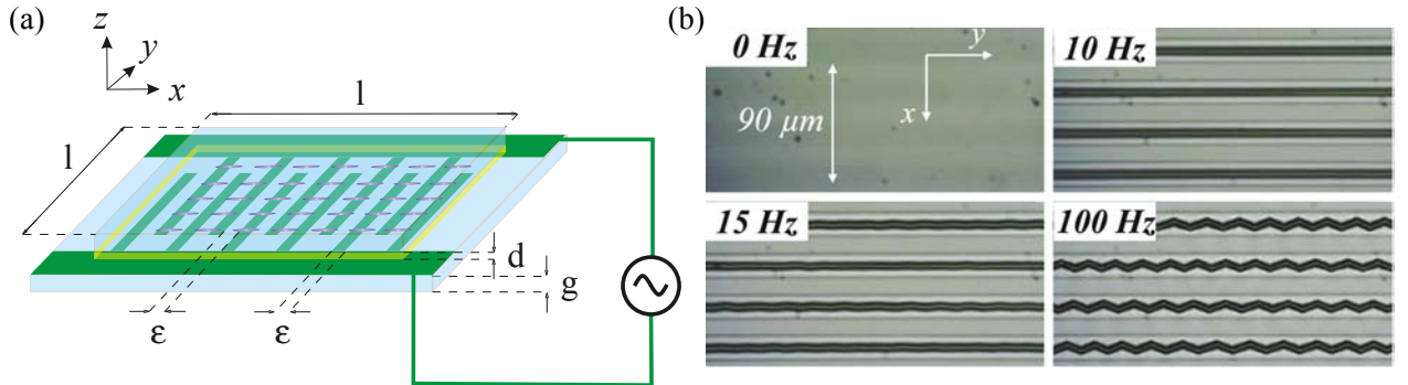
Figure 2.25: (a) Schematic representation of the liquid crystal IPS cell, connected to a generator. (b) Zig-zag instability exhibited by a nematic liquid crystal filled in this cell.
