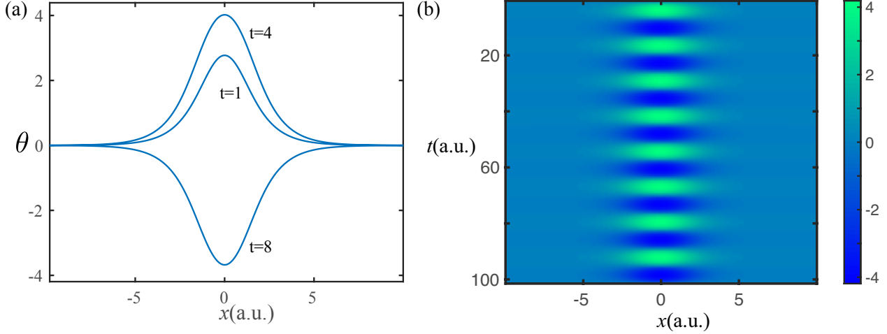
Figure 2.14: Temporal evolution of breather solution. (a) Spatial profile evolution for different times. (b) Corresponding spacetime diagram. We have used \Omega = 0.5 .
