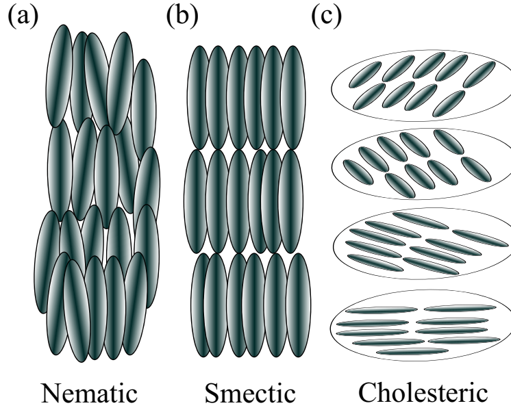
Figure 2.24: Different liquid crystal phases: nematic, smectic and cholesteric.
