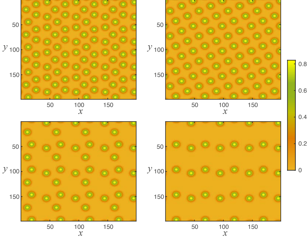
Figure 4.9: Different equilibrium configuration of two dimensional localized structures. The parameters used were \eta = 0.12, \kappa = 0.6, \Delta = 0.02, \Gamma = 0.5, \alpha = 0.125, dx = dy = 0.3 and dt = 0.001 , with periodic boundary conditions.
