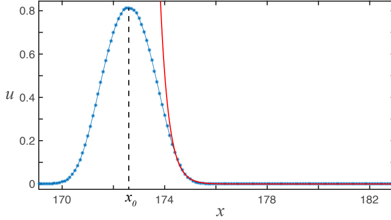
Figure 4.1: One dimensional localized structure profile. The parameters used are \eta = 0.17, \kappa = 0.8, \Delta = 0.02, \Gamma = 0.5 and \alpha = 0.13 . The red line corresponds to the exponential fitting, using Eq. (4.3). For this case the theoretical value of \gamma is 2.91 and from the fitting 3.06. The coefficient of determination results R^2 = 0.9978 .
