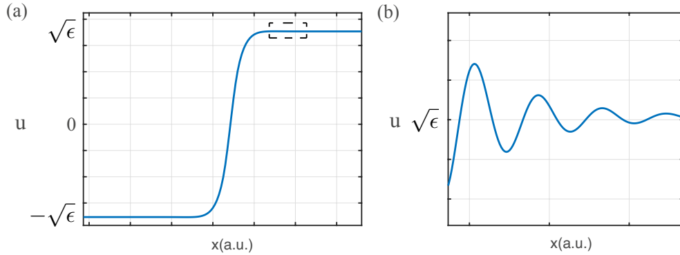
Figure 3. (a) Profile of the stationary flaming kink solution of equation (8). The dashed rectangle corresponds to a zoom showed in (b). (b) Stationary evanescent waves present in the kink solution.
