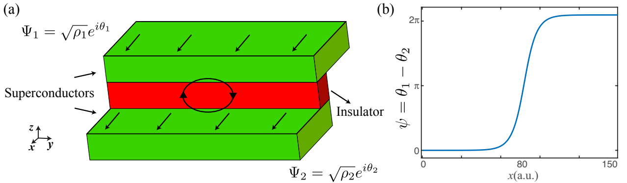
Figure 3.14: (a) Schematic representation of a Josephson junction. The green layers represent superconductors and the red one an insulator material. The terms \Psi_1 and \Psi_2 account for the macroscopic wavefunctions in every layer. (b) Kink (or fluxon) solution of the phase difference \psi = \theta_1 - \theta_2 .
