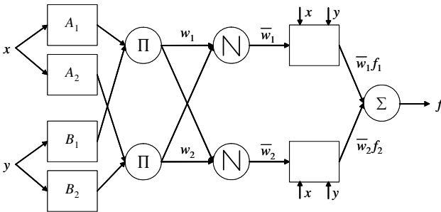
Fig. 3. ANFIS architecture [7].
